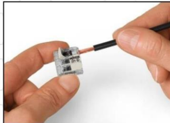
Termination: Lift the lever open the clamping unit and insert a stripped conductor
