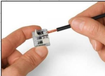
Strip conductor to 11mm
